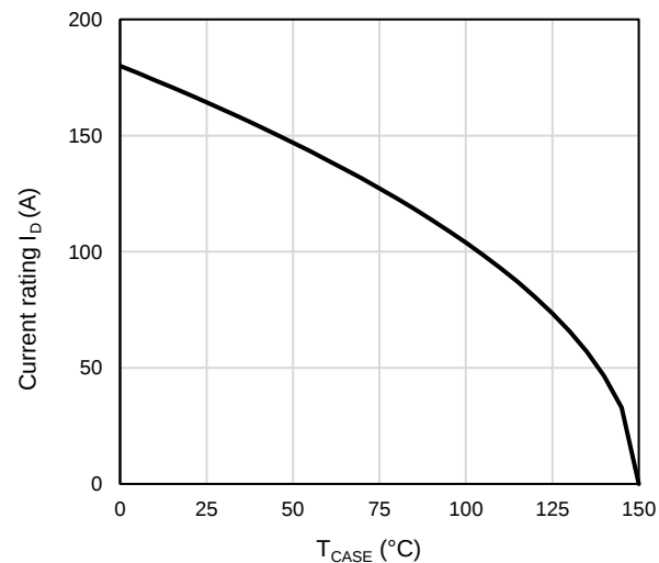
Figure 12: Current De-rating
